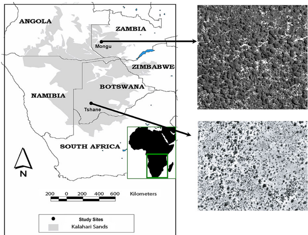
Fig. 1 Sampling locations and vegetation characteristics along the KT. The satellite images of each site are IKONOS (Tshane) and Quickbird (Mongu)
