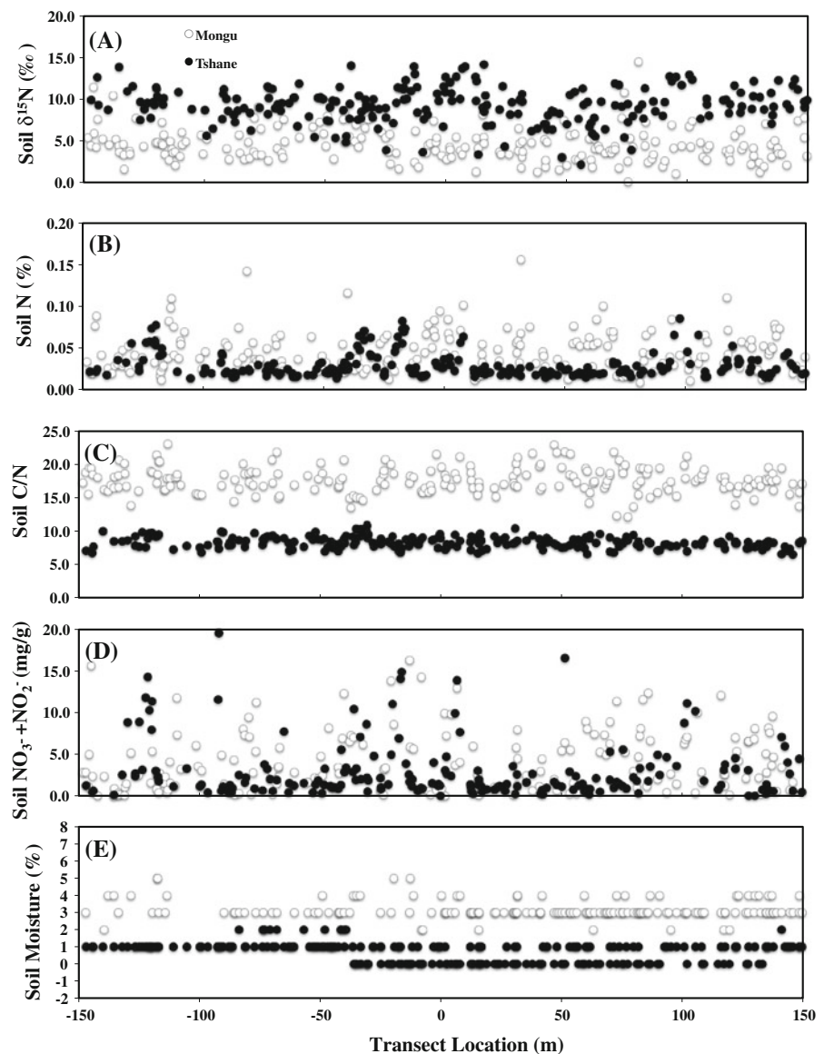
Fig. 2 Ecosystem-scale variations of \delta^{15}\text{N} (a), soil %N (b), soil C/N (c), soil \text{NO}_3^- + \text{NO}_2^- (d) and soil moisture (e) at Tshane and Mongu. The %N, C/N and \text{NO}_3^- + \text{NO}_2^- data have been reported in Okin et al. (2008) and were used here to facilitate the interpretations of soil \delta^{15}\text{N} spatial pattern
