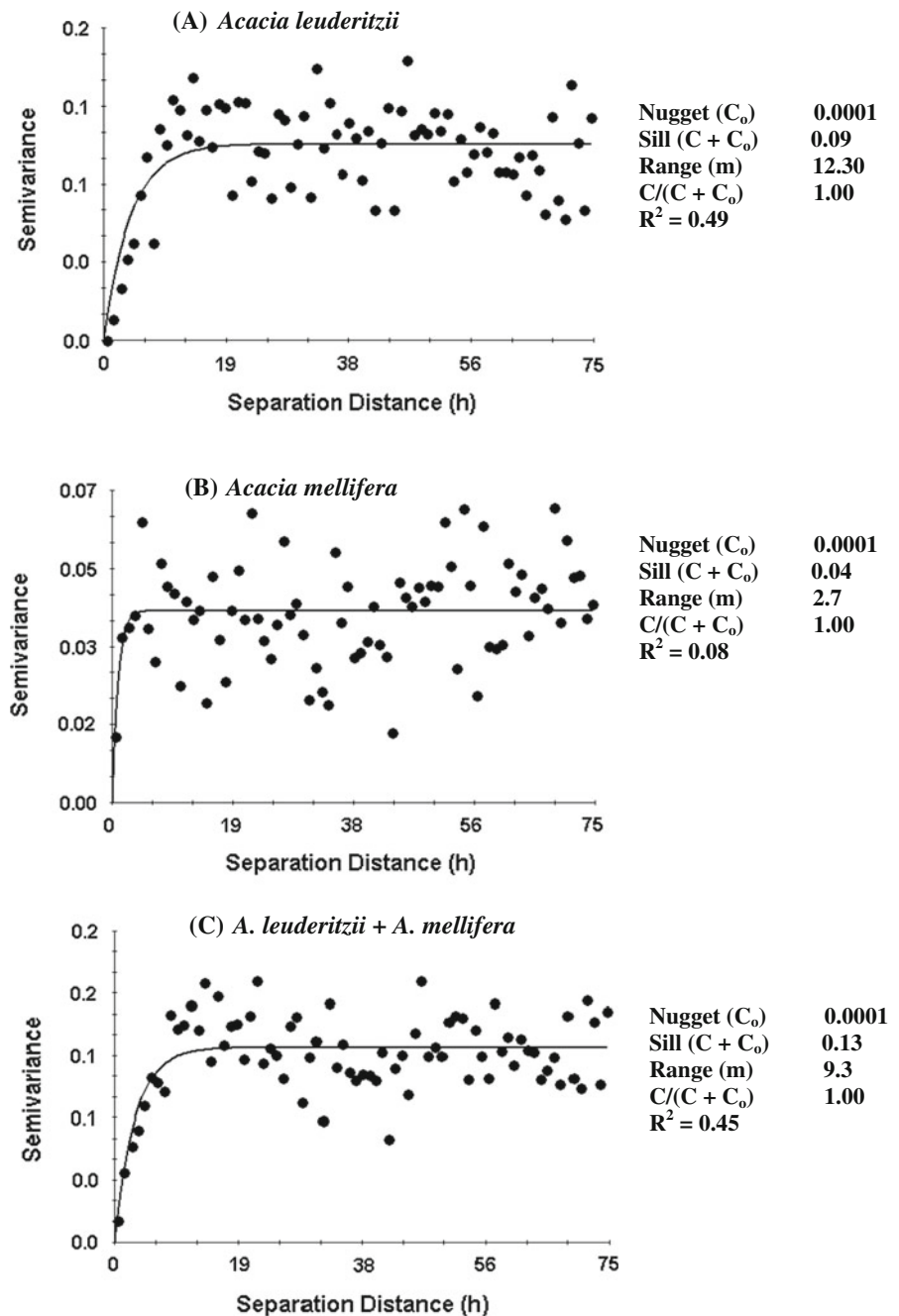
Fig. 5 Semivariograms of Acacia leuderitzii alone (a), Acacia mellifera alone (b) and the combination of the two (c) at Tshane. The summary of semivariogram model parameters is reported on the right
