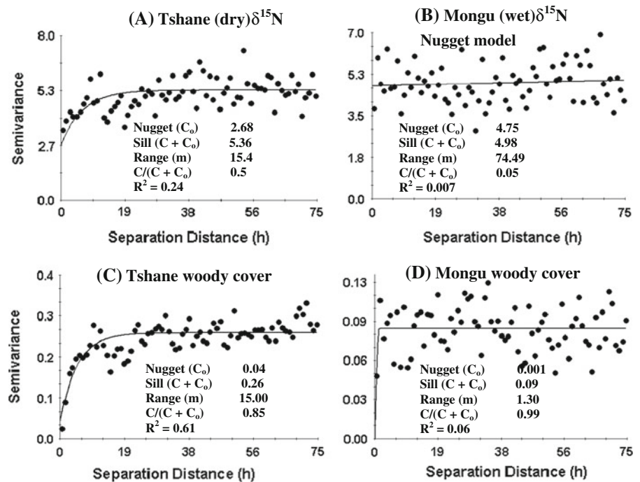
Fig. 3 Semivariograms of \delta^{15}\text{N} at Tshane (a), Mongu (b), and semivariograms of woody cover at Tshane (c) and Mongu (d) along the KT. The summary of semivariogram model parameters is reported under the curve. Proportion structural variation ( C/(C + C_0) ) is used as an index of the magnitude of spatial dependence
