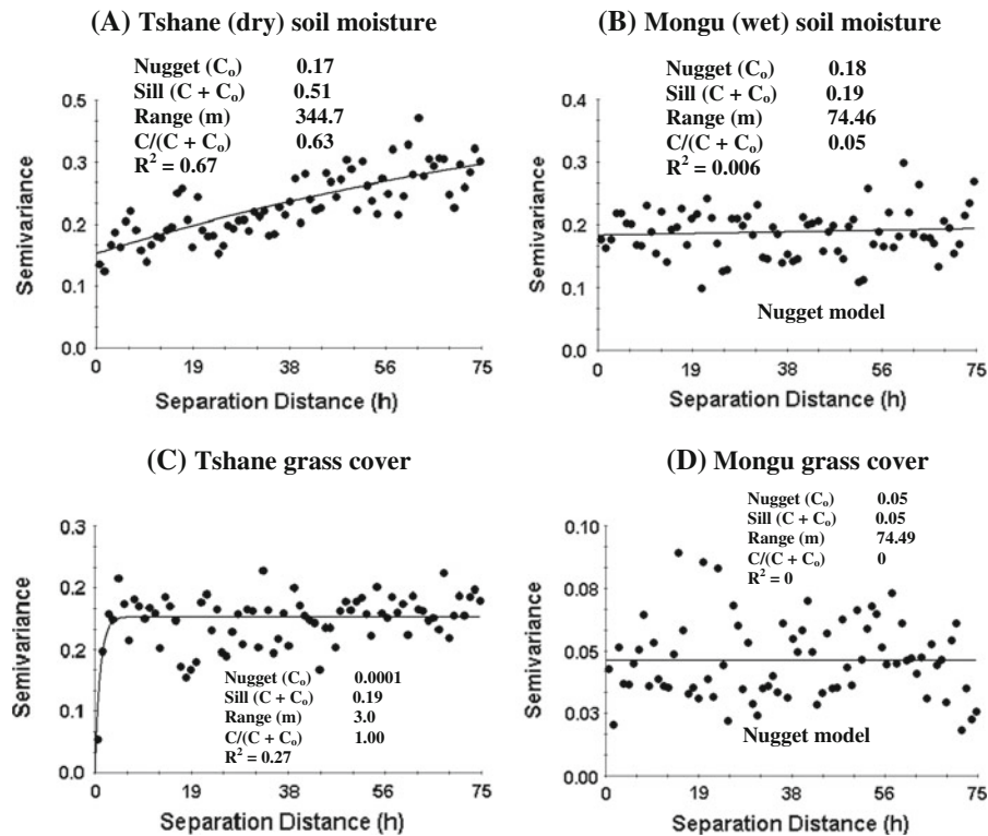
Fig. 4 Semivariograms of soil moisture at Tshane (a), Mongu (b), and semivariograms of grass cover at Tshane (c) and Mongu (d) along the KT. The summary of semivariogram model parameters is reported close to the curve
